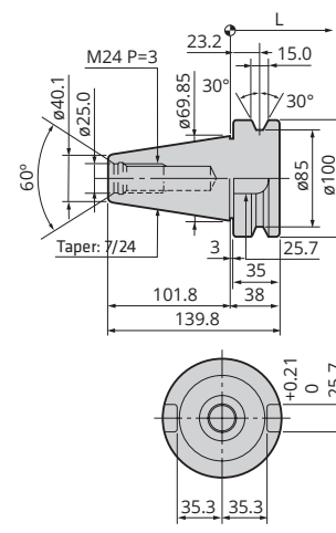
BT50
