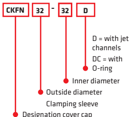
Cover cap for direct clamping: D, DC (CKFN-D, DC)
