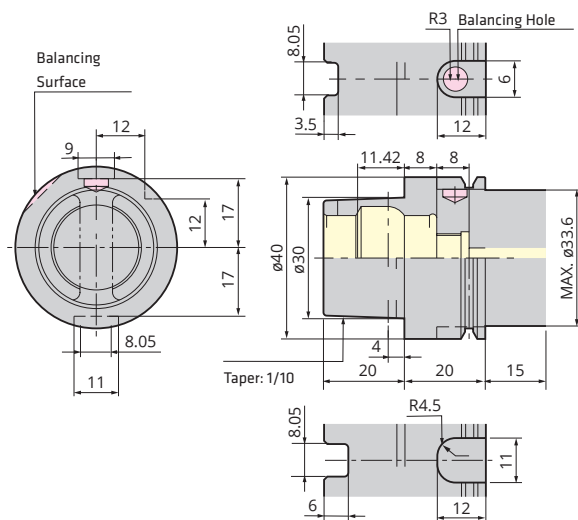
HSK40A (ISO 12164-1)
