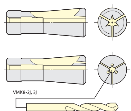
Cutting tool without internal cooling
