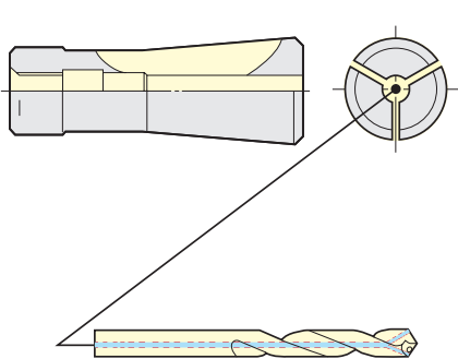
Cutting tool with internal cooling
