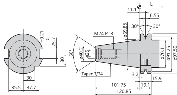
BT50
