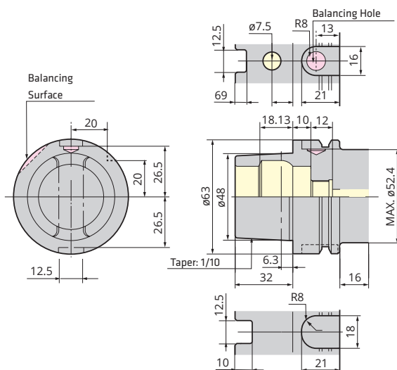
IT40 (ISO7388, DIN69871-'85)
