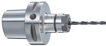
Slim Chuck
