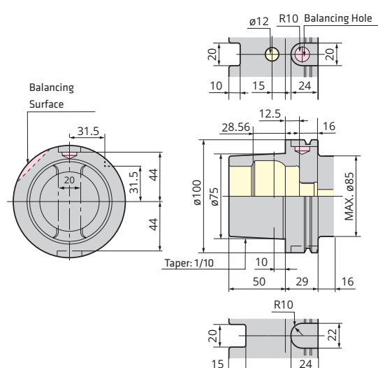
IT50 (ISO7388, DIN69871-'85)
